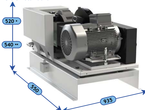
HOSPITAIR® SCROLAIR G version standard
